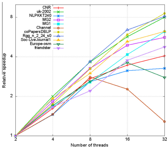
Fig. 7. Speedup charts for our parallel implementation, Grappolo . The chart on left shows the relative speedup of the parallel implementation using the 2-thread run as the reference. The chart on the right shows the absolute speedup – i.e., relative to the serial Louvain implementation [10]. All speedups are calculated using the baseline + VF + Color implementation of Grappolo . Note that in the absolute speedup chart, curves for Europe-osm and friendster are not shown because the serial Louvain implementation failed to complete on these two inputs.
