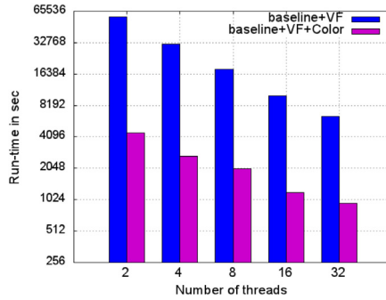
(k) Input: friendster
