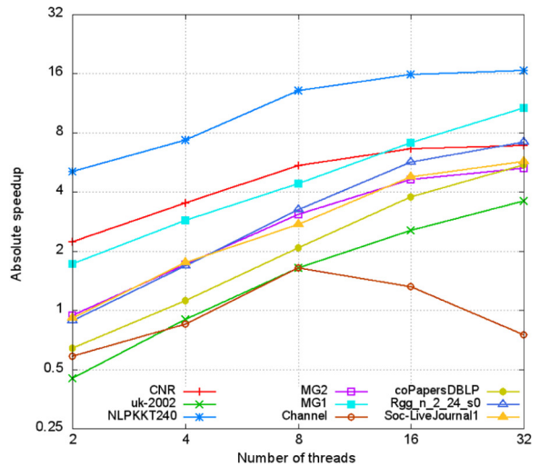
Fig. 7. Speedup charts for our parallel implementation, Grappolo . The chart on left shows the relative speedup of the parallel implementation using the 2-thread run as the reference. The chart on the right shows the absolute speedup – i.e., relative to the serial Louvain implementation [10]. All speedups are calculated using the baseline + VF + Color implementation of Grappolo . Note that in the absolute speedup chart, curves for Europe-osm and friendster are not shown because the serial Louvain implementation failed to complete on these two inputs.
