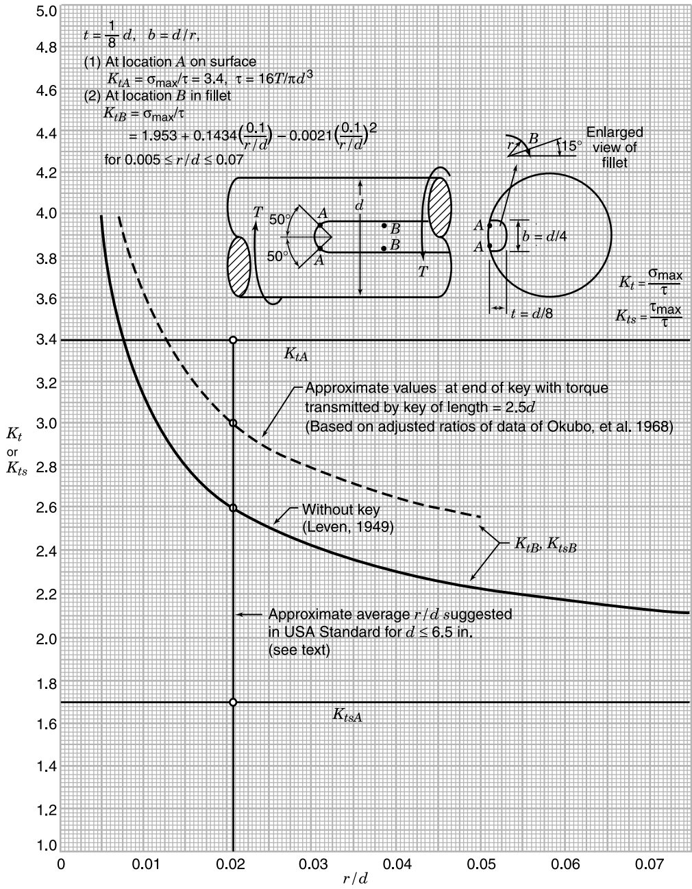
Chart 5.2 Stress concentration factors K_r, K_s for a torsion shaft with a semicircular end keyseat (Leven 1949; Okubo et al. 1968).
