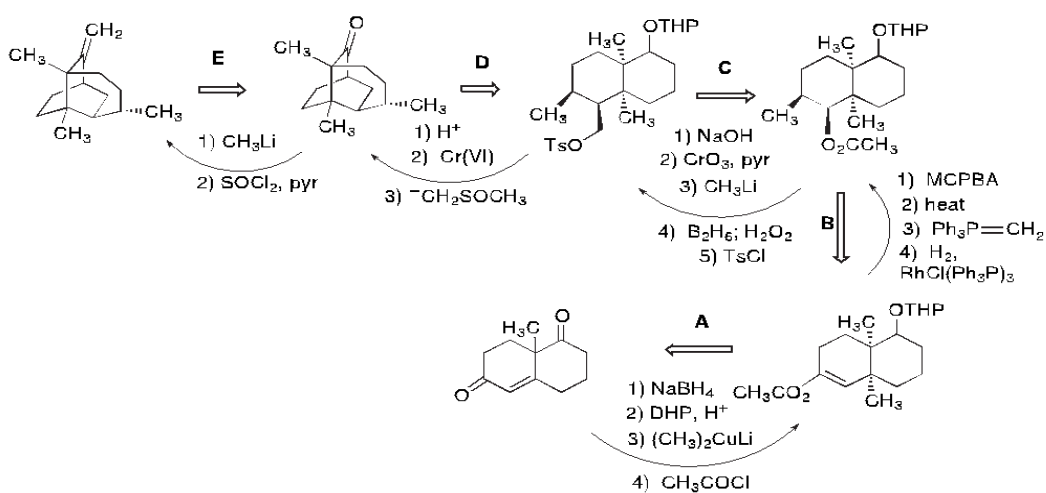
Scheme 13.P9a-1. Seychellene Synthesis: E. Piers, R. W. Britton, and W. de Waal a
