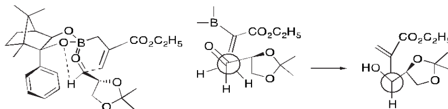
transition structure for anti product from S -aldehyde
