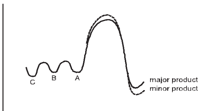
Fig. 4.P23B. Representation of energy profile for iodolactonization of 23-B .
