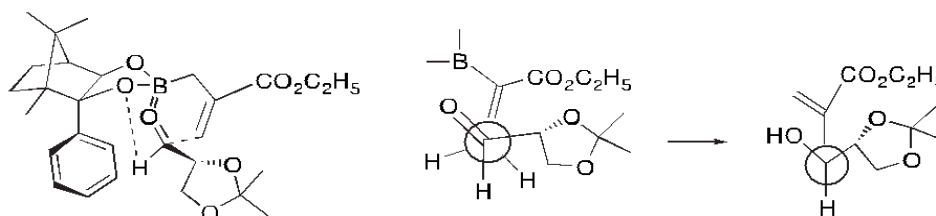
transition structure for syn product from R -aldehyde
