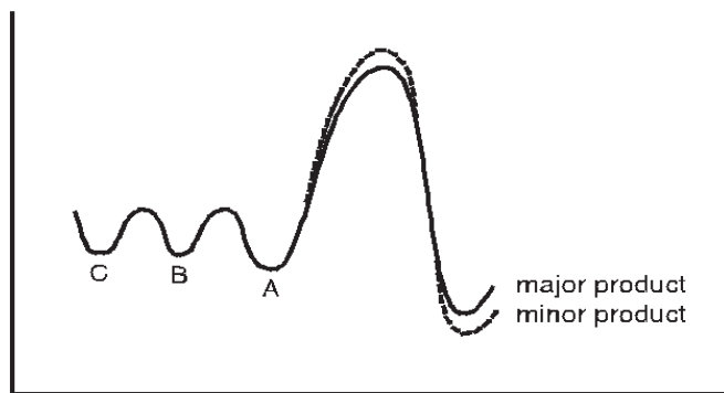
Fig. 4.P23A. Representation of energy profile for iodolactonization of 23-A . In compound, the additional substituent makes the disubstituted double bond more reactive. This cyclization occurs from a conformation ( A 1 ), which is not the most stable but proceeds through a lower-energy intermediate because of the activation by the methyl group.
