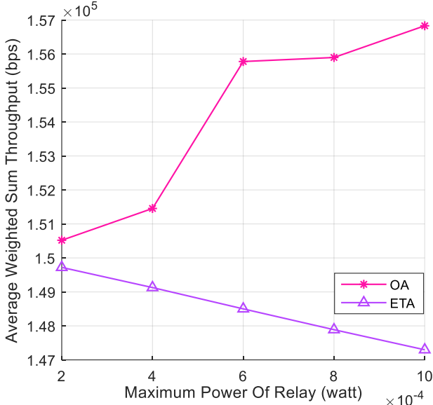
Fig. 6: Comparison of AWST diagrams in terms of P_r^{max} for OA and ETA modes.
