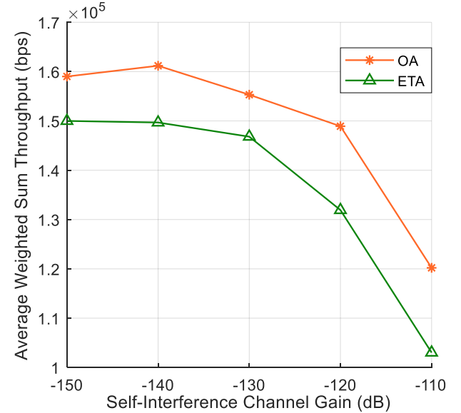
Fig. 5: Comparison of AWST diagrams in h_{rr} for OA and ETA modes.
